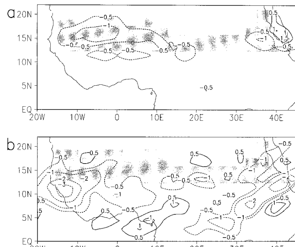
FIG. 6. JAS mean changes in components of the water budget due to degradation of region DN. The degraded area is shaded. Contours are drawn at \pm 0.5, 1, 2, and 3 \text{ mm day}^{-1} : (a) evaporation and (b) vertically integrated moisture flux convergence.
